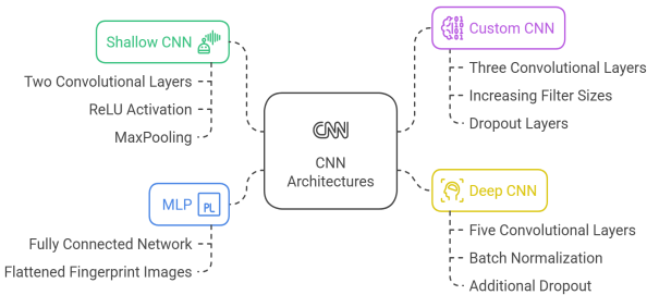
Fig. 3. CNN Architectures Used
